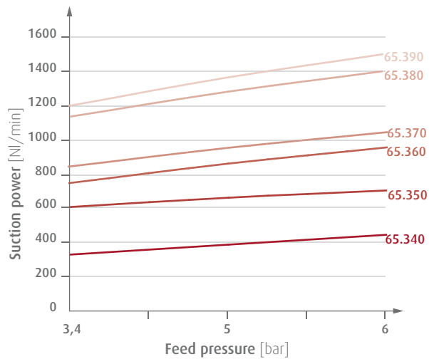
> Suction power against feed pressure
