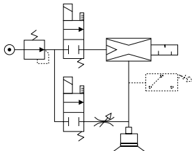
Ejector with controlled blow-off-function EMM__X__AV__
