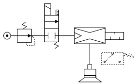
Ejector with blow-off-function EMM__X__EV__
